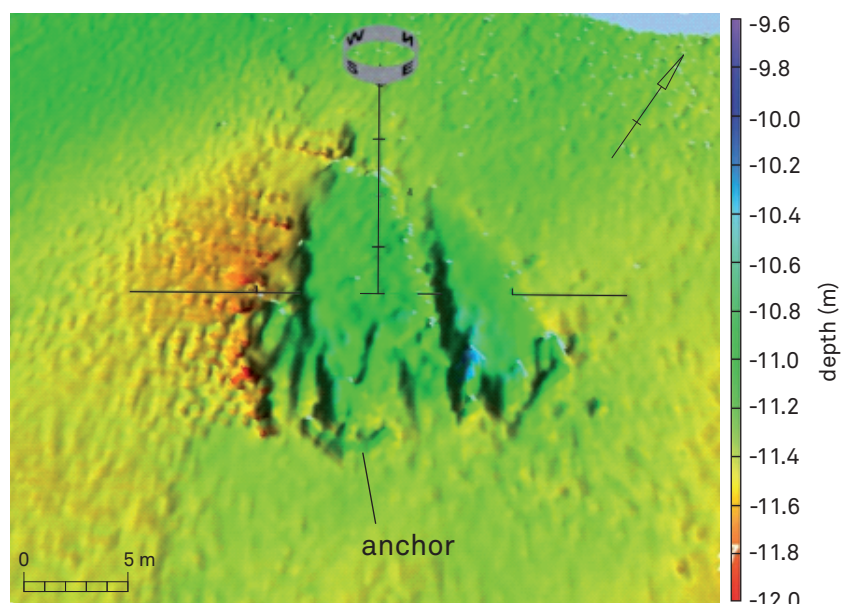
FIG. 11 Multibeam image acquired in 2007 over the Buiten Ratel wreck site (Flemish Hydrography). The two large wreck pieces can be clearly observed.
